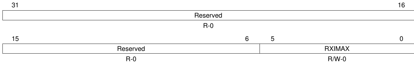
Figure 28-26. EMAC Control Module Receive Interrupts Per Millisecond Register (C0RXIMAX)
