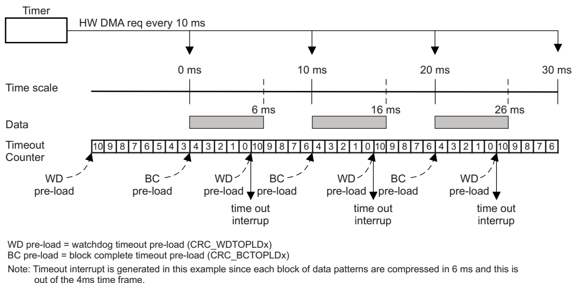
Figure 14-7. Timeout Example 2
