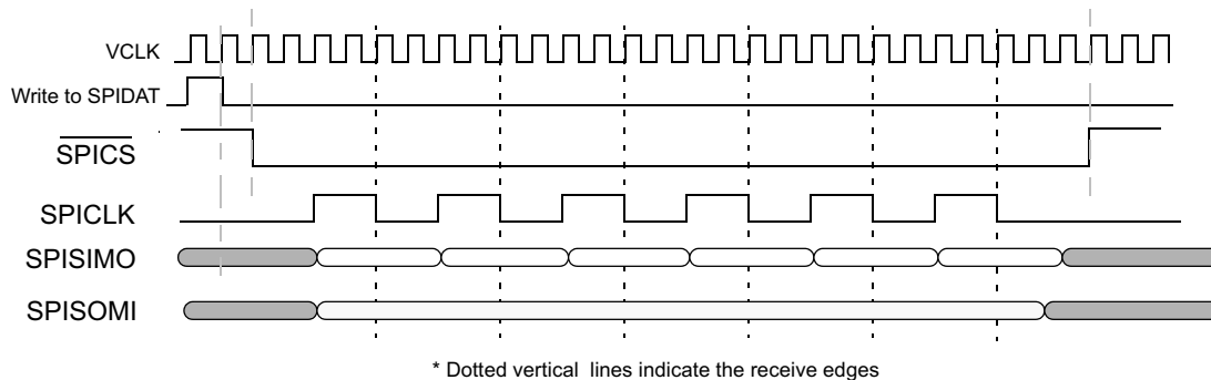
Figure 24-82. SPI/MibSPI Pins During Master Mode 4-pin with \overline{\text{SPICSS}} Configuration
