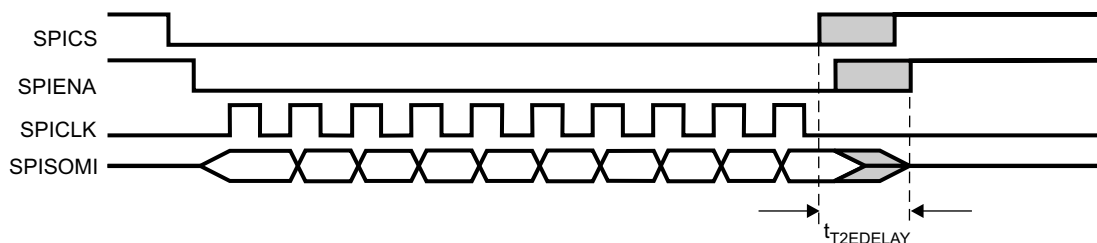
Figure 24-47. Transmit-Data-Finished-to-ENA-Inactive-Timeout
