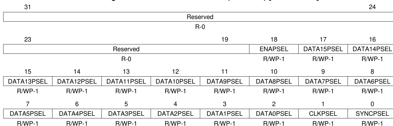
Figure 30-30. DMM Pin Control 8 (DMMP8) [offset = 8Ch]
