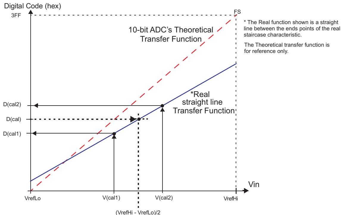
Figure 19-12. Mid-point Value Calculation
