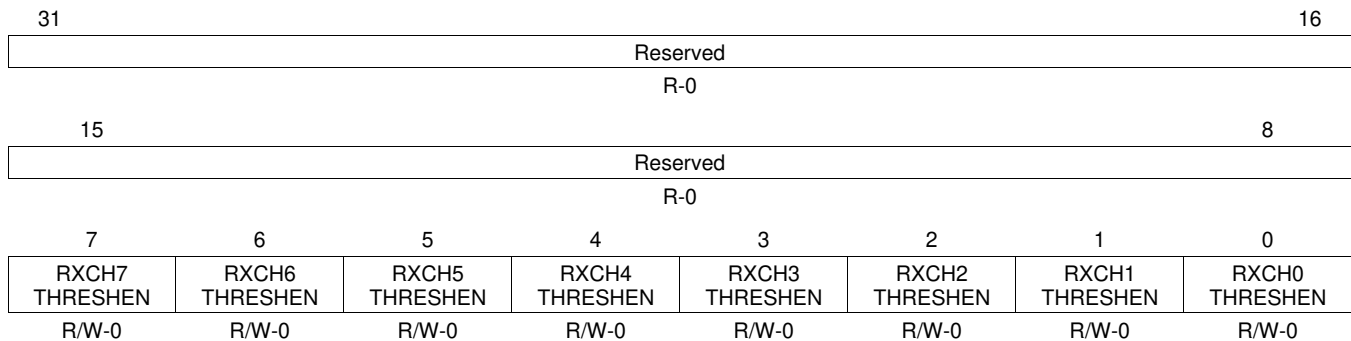
Figure 28-18. EMAC Control Module Receive Threshold Interrupt Enable Register (C0RXTHRESHEN)
