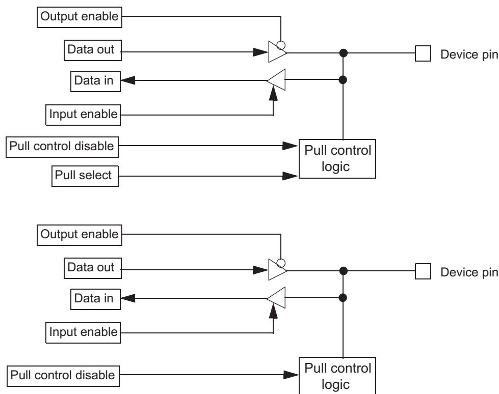
Figure 25-60. GPIO Functionality
