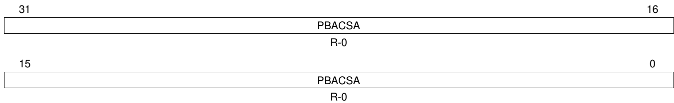
Figure 16-65. Port B Active Channel Source Address Register (PBACSAADDR) [offset = 198h]
