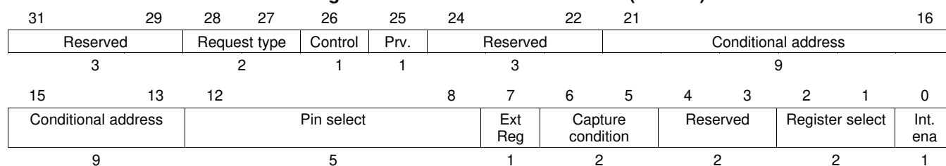
Figure 20-187. WCAP Control Field (C31:C0)
