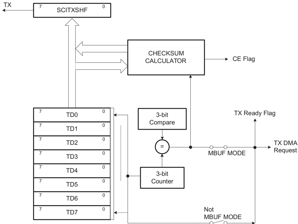
Figure 25-9. Transmit Buffers
