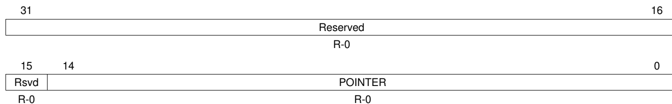
Figure 30-16. DMM Direct Data Mode Pointer Register (DMMDDMPT) [offset = 24h]
